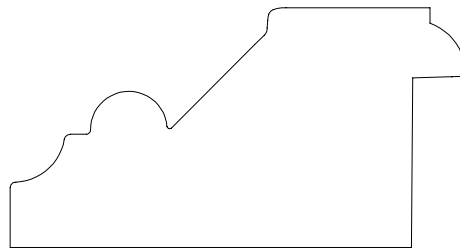
BACKBAND 6238 1 1/4" X 2 3/8" 1/4" X 7/8" THROAT
