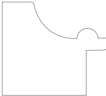
BACKBAND 6188 1 11/16" X 1 7/8" 3/8" X 13/16" THROAT
