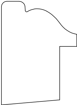
BACK BAND 61008 1 3/8" X 1" OLD 100
