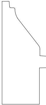
BACKBAND 61881 1 7/8" x 13/16" 1/8" x 5/8" THROAT
