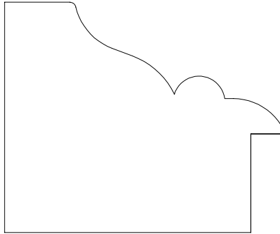
BACKBAND 6213 1 3/4" X 2 1/8" 1/4" X 3/4" THROAT
