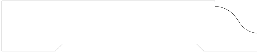
BASE 235011 11/16" X 3 1/2"
