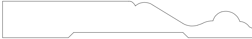
BASE 24258 5/8" x 4 1/4"
