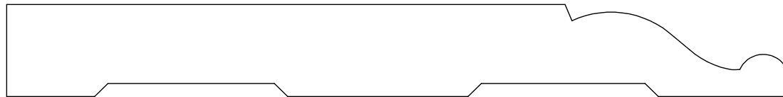
BASE 252513 5/8" X 5 1/4"
