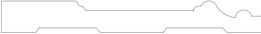
BASE 25136 5/8" X 5 1/8"
