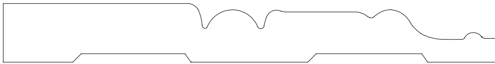
BASE 252532 5/8" X 5 1/4"
