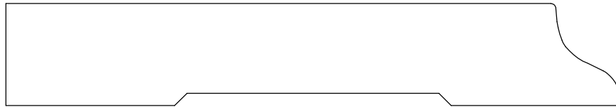
BASE 245040 3/4" x 4 1/2"
