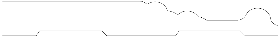
BASE 250013 5/8" X 5"
