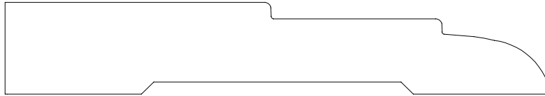
BASE 24134 11/16" x 4 1/8"
