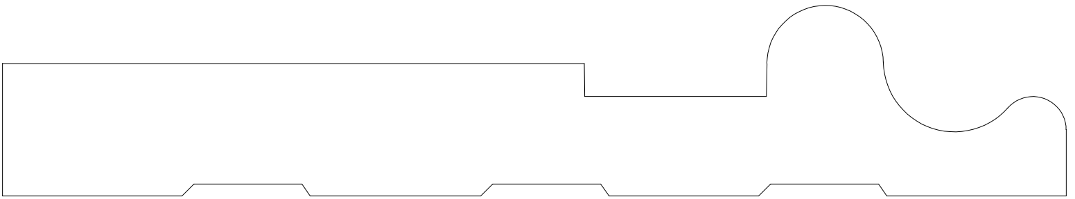
BASE 28005 1 7/16" X 8"
