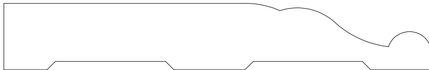
BASE 24251 11/16" X 4 1/4"
