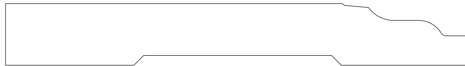
BASE 245013 5/8" X 4 1/2"
