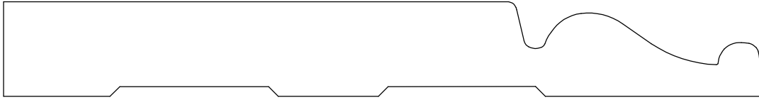
BASE 25505 11/16" X 5 1/2"
