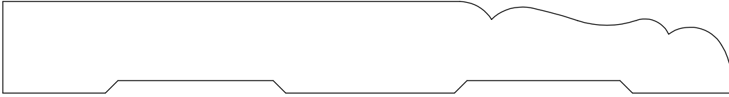
BASE 252510 5/8" X 5 1/4"
