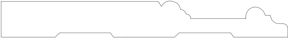
BASE 260012 3/4" x 6"
