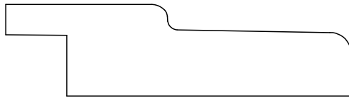
BASE CAP 22131 9/16" X 2 1/8"
