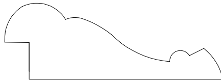
BASE CAP 22254 3/4" X 2 1/4" ( 3/8" X 1/4" NOTCH )
