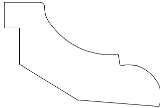
BASE CAP 21883 11/16" X 1 15/16"
