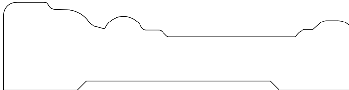
CASING 135044 7/8" X 3 1/2"
