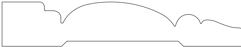
CASING 140014 3/4" X 4"
