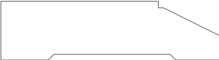
CASING 1350109 15/16" X 3 1/2"
