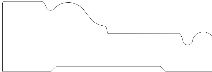
CASING 137511 1 1/4" X 3 3/4"
