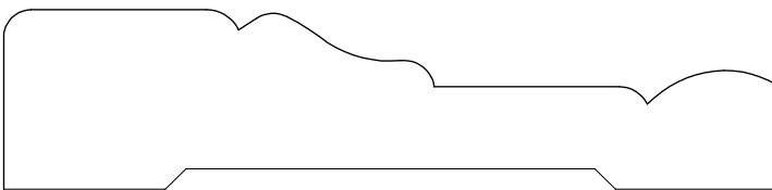
CASING 1350110 13/16" X 3 1/2"
