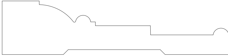
CASING 14503 1 1/16" X 4 1/2"
