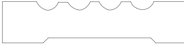
CASING 1331 3/4" X 3 5/16"
