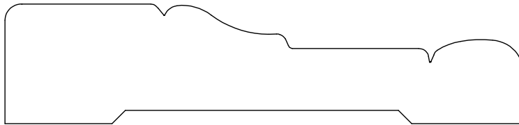
CASING 1350103 13/16" X 3 1/2"
