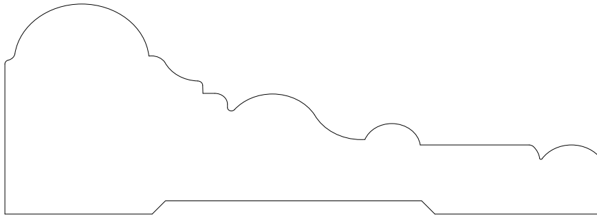
CASING 14253 1 1/2" X 4 1/4"
