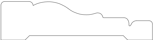
CASING 130010 3/4" X 3" OLD 300-1
