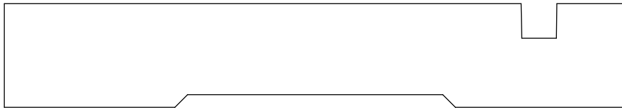
CASING 145010 3/4" X 4 1/2"
