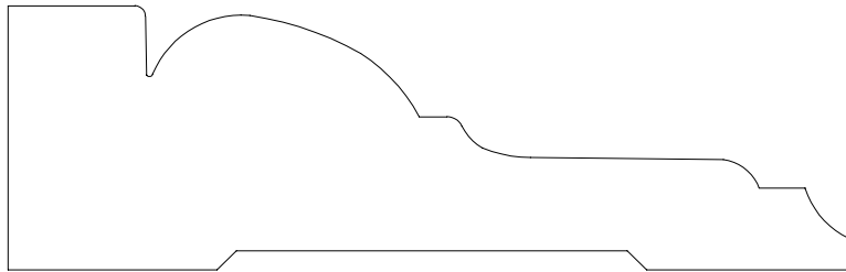
CASING 140032 1 1/4" X 4"
