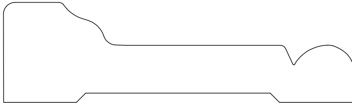
CASING 135029 1" X 3 1/2" OLD 1350-2
