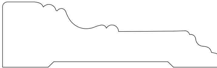
CASING 135020 1 1/16" X 3 1/2"
