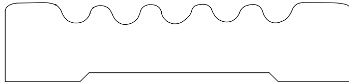
CASING 13634 13/16" X 3 9/16"
