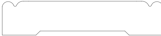
CASING 1350170 3/4" X 3 1/2"
