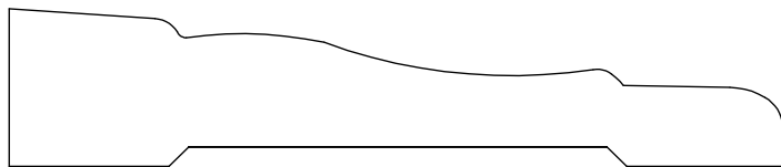
CASING 135023 1 1/16" X 3 1/2" OLD 350-2 (SIMILAR TO MDF 444M)
