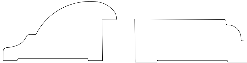
CASING 1200 1" X 2" OLD 200-0-1 CASING 12001 3/4" X 2" OLD 200-0-2
