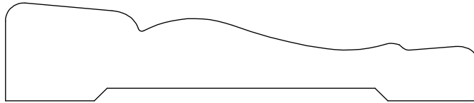
CASING 13258 11/16" X 3 1/4" OLD 325-0 (SIMILAR TO MDF444L)
