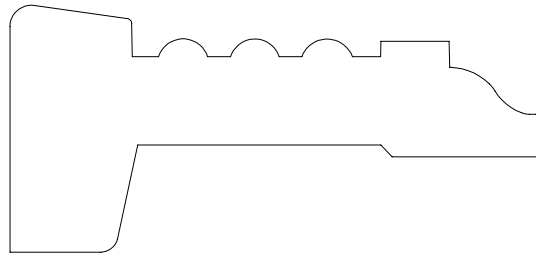
CASING 12811 1 5/16" X 2 3/4"
