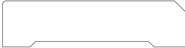
CASING 130020 3/4" X 3"
