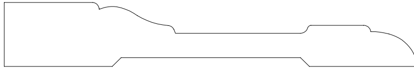
CASING 142525 11/16" X 4 1/4"
