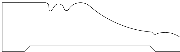
CASING 127518 3/4" X 2 3/4"
