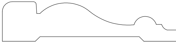
CASING 132515 3/4" X 3 1/4" (SIMILAR TO MDF 9003)
