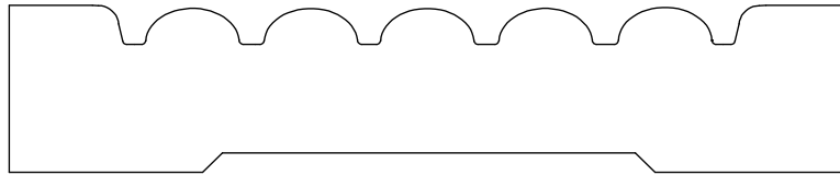
CASING 13751 3/4" X 3 3/4"
