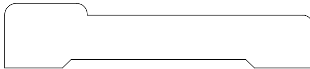
CASING 132529 11/16" X 3 1/4"
