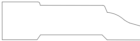
CASING 125051 11/16" X 2 1/2"
