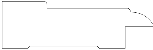
CASING 126310 13/16" X 2 5/8" ( 1/2" X 3/8" KNOTCH)
