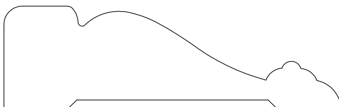
CASING 132512 1" X 3 1/4" (SIMILAR TO MDF 3122)
