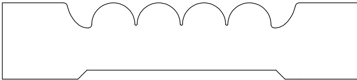
CASING 1350107 3/4" X 3 1/2"
