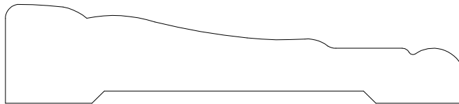
CASING 132510 11/16" X 3 1/4" (SIMILAR TO MDF 445M)
