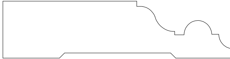
CASING 140028 1" X 4"
