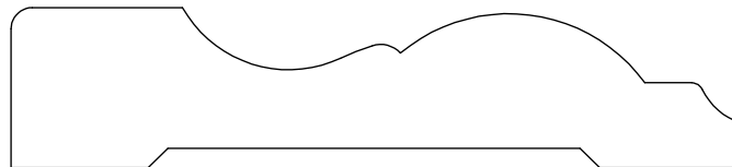
CASING 132517 3/4" X 3 1/4" (SIMILAR TO MDF 8063)
