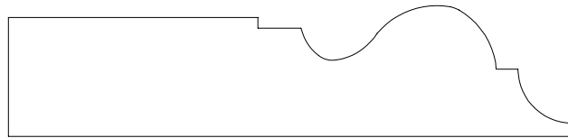
CASING 132541 3/4" X 3 1/4"
