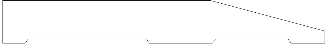
CASING 1650 7/8" X 6 1/2"
