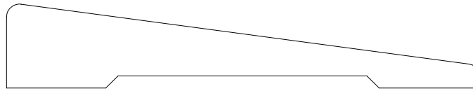
CASING 1350161 5/8" X 3 1/2"
