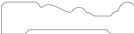
CASING 127511 11/16" X 2 3/4"
