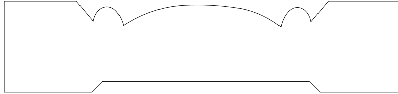
CASING 135091 13/16" X 3 1/2"
