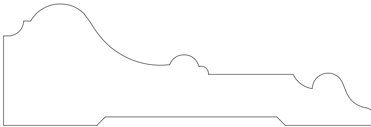
CASING 14006 1 5/16" x 4"
