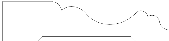
CASING 1350172 13/16" X 3 1/2"
