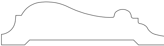
CHAIR RAIL 5288 3/4" X 2 7/8"
