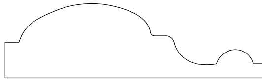
CHAIR RAIL 52756 3/4" X 2 3/4"
