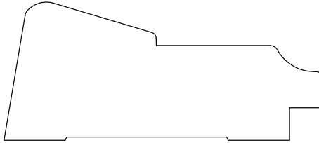
CHAIR RAIL 52441 1 1/16" X 2 7/16"
