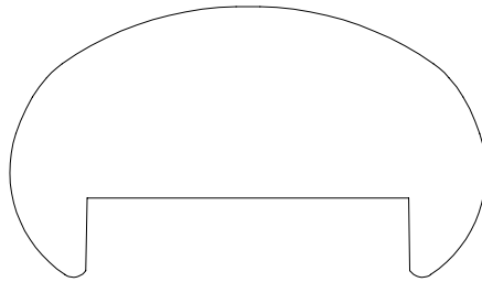
HANDRAIL 922515 1 9/32 X 2 1/4"
