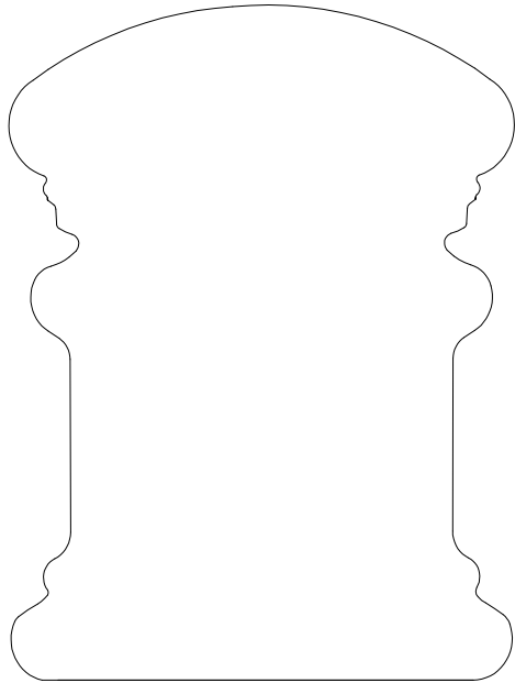
HANDRAIL 93002 3" X 4"
