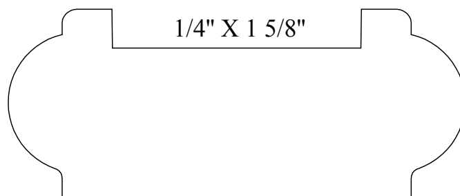
SHOERAIL 930016 1 1/4" X 3"
