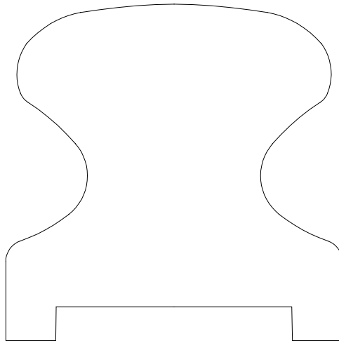
HANDRAIL 925031 2 1/2" X 2 1/2" ( 1 3/4" PLOW )
