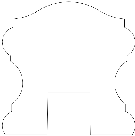
HANDRAIL 92385 2 3/8" X 2 3/8" ( 3/4" X 3/4" PLOW )
