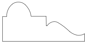
PANEL MOULD 71446 11/16" X 1 7/16"
