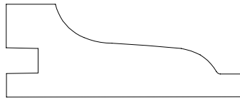
PANEL MOULD #717523 5/8" x 1 3/4"
