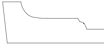
PANEL MOULD 717525 23/32" X 1 3/4"
