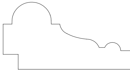
PANEL MOULD #72131 1 1/8" x 2 1/8"
