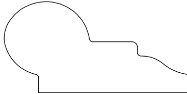
PANEL MOULD 91756 7/8" X 1 3/4"
