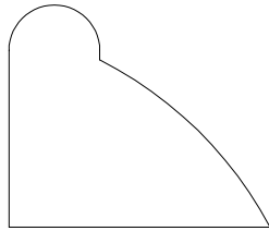
PANEL MOULD 712526 1 1/16" X 1 1/4"
