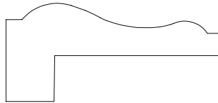
PANEL MOULD 716318 3/4" X 1 5/8" THROAT 3/8"
