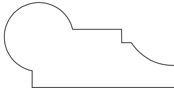
PANEL MOULD 71639 13/16" X 1 5/8"
