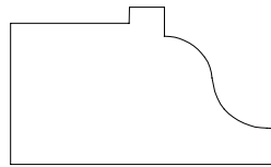
PANEL MOULD 712529 3/4" X 1 1/4"
