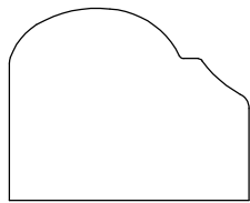
PANEL MOULD 911314 15/16" X 1 1/8"
