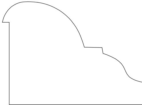
PANEL MOULD 7257 1 7/8" X 2 9/16" 1/8" X 1 1/2" THROAT
