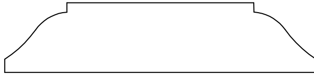
PANEL MOULD 72504 9/16" X 2 1/2"
