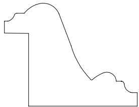
PANEL MOULD 713817 1 1/8" x 1 3/8" 3/4" THROAT
