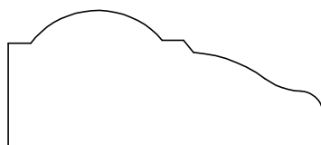
PANEL MOULD 71441 5/8" X 1 7/16"
