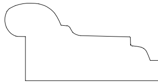
PANEL MOULD #716315 13/16" x 1 5/8"
