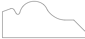
PANEL MOULD 715033 21/32" X 1 1/2"
