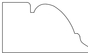
PANEL MOULD 715022 7/8" X 1 1/2"
