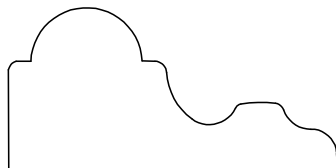
PANEL MOULD 7144 11/16" X 1 7/16" OLD 1384
