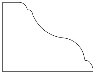
PANEL MOULD 71386 1 1/16" X 1 3/8"
