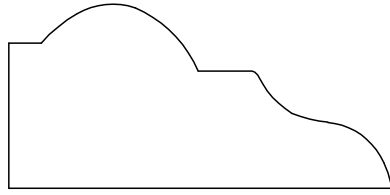
PANEL MOULD 7169 13/16" X 1 11/16"
