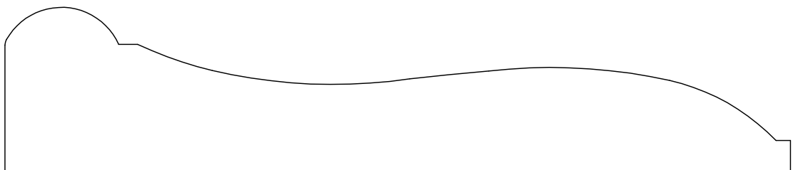
PANEL MOULD 7500 1 1/16" X 5"
