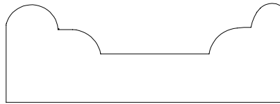
PANEL MOULD 72062 3/4" X 2 1/16"
