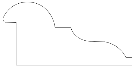
PANEL MOULD 72257 1 5/64" X 2 7/32"
