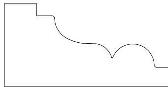
PANLEL MOULD 717530 7/8" X 1 3/4"
