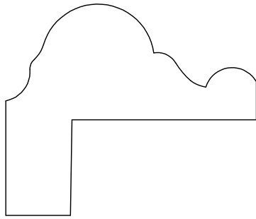
PANEL MOULD 71636 1 3/8" X 1 5/8"
