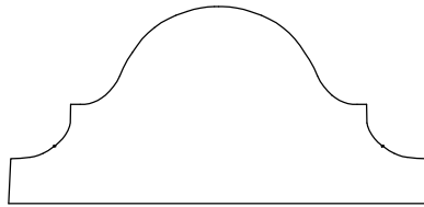
PANEL MOULD 720023 15/16" X 2"
