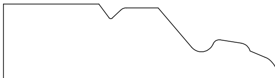
PANEL MOULD 72503 11/16" X 2 1/2"
