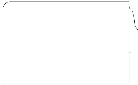
PANEL MOULD 92384 1 13/32" X 2 11/32"
