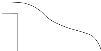
PANEL MOULD 716311 13/16" X 1 5/8"
