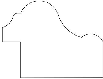
PANEL MOULD 71383 11/16" X 1 3/8"
