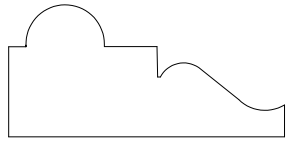
PANEL MOULD 71445 11/16" X 1 7/16"
