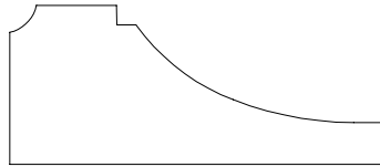
PANEL MOULD 717526 3/4" X 1 3/4"
