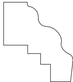
PANEL MOULD 71007 3/4" X 1 1/2"
