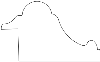
PANEL MOULD 71503 7/8" X 1 1/2"
