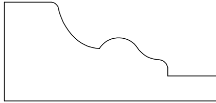
PANEL MOULD 717511 13/16" X 1 13/16"
