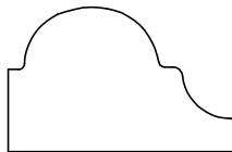
PANEL MOULD 70881 9/16" X 7/8"
