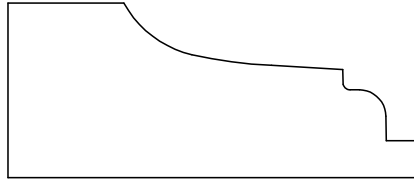
PANEL MOULD 717510 3/4" X 1 3/4"
