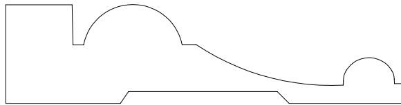
PANEL MOULD 73002 3/4" X 3"
