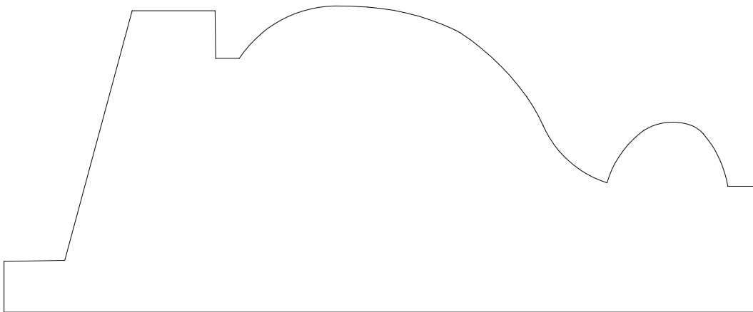
PANEL MOULD 955033 2 1/4" X 5 1/2"
