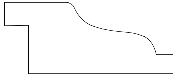
PANEL MOULD 717524 3/4" X 1 3/4" ( 1/2" THROAT)
