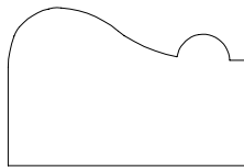
PANEL MOULD 71137 3/4" X 1 1/8"
