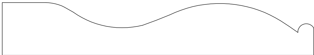
PANEL MOULD 7475 13/16" X 4 3/4"
