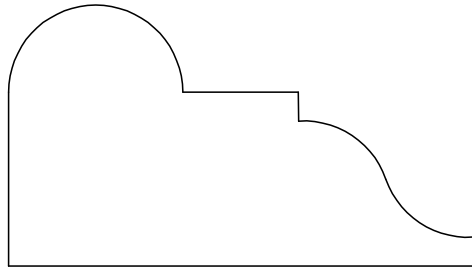
PANEL MOULD 720017 1 1/8" X 2"
