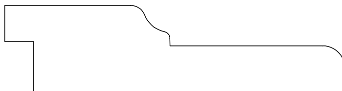
PANEL MOULD 9293 3/4" X 2 15/16"
