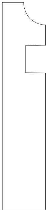
PANEL MOULD 93561 3/4" x 3 1/2"
