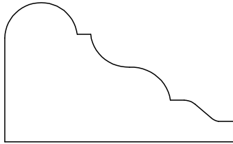
PANEL MOULD 71443 7/8" X 1 7/16"
