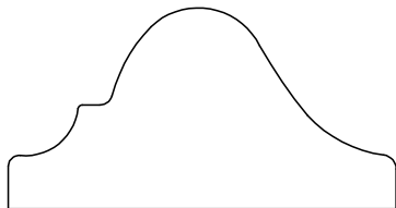
PANEL MOULD 715010 3/4" X 1 1/2"
