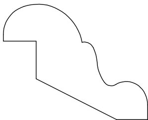
PANEL MOULD 716312 11/16" X 1 5/8"
