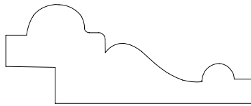
PANEL MOULD #9188 3/4" x 1 7/8"
