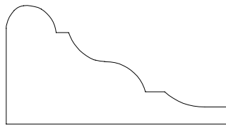
PANEL MOULD 716319 7/8" X 1 5/8"
