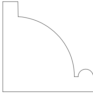
PANEL MOULD #715026 1 1/2" x 1 1/2"
