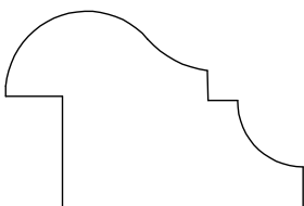
PANEL MOULD 71321 7/8" X 1 5/16"
