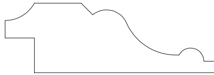
PANEL MOULD 72256 3/4" x 2-1/4"
