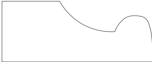
PANEL MOULD 7288 1 1/8" X 2 7/8"
