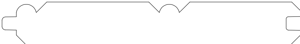
PLANKING 9525_11 3/4" X 5 1/4" LAYS 5"
