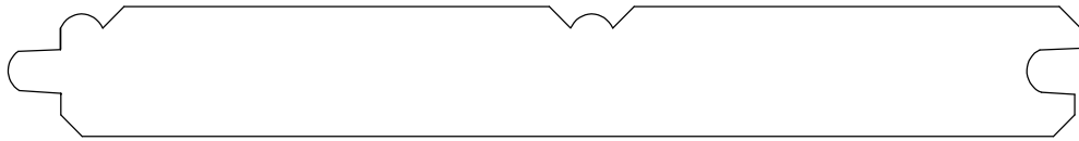
PLANKING 951302 5/8" X 5 1/8" LAYS 4 7/8"
