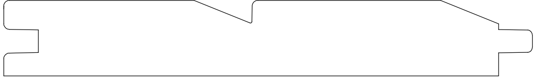
PLANKING 9569 13/16" X 5 11/16" LAYS 5 5/16"
