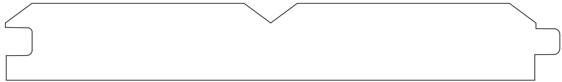
PLANKING 9538 3/4" X 5 3/8" LAYS 5 1/8"
