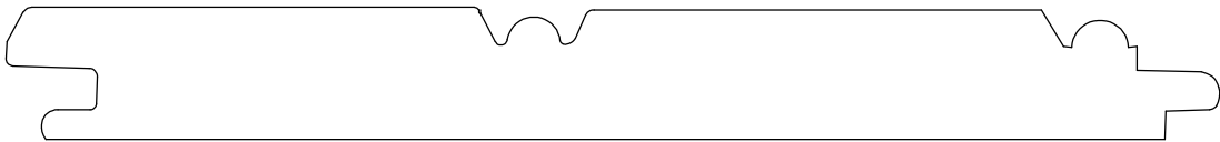
PLANKING 9425 7/16" X 4 1/4" LAYS 4"
