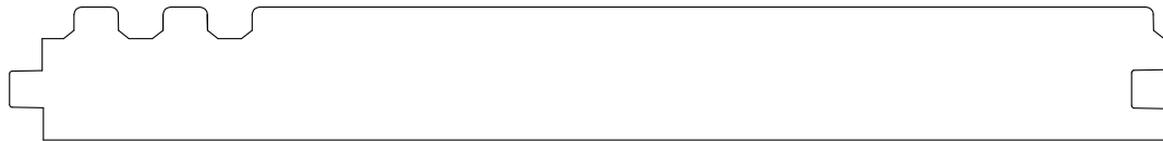
PLANKING 97502 3/4" X 6 1/2" LAYS 6 1/4"
