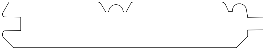
PLANKING 935022 5/8" X 3 9/16" LAYS 3 5/16"
