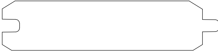
PLANKING 93257 3/4" X 3 1/4" LAYS 3"
