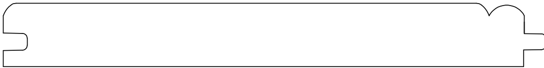
PLANKING 942512 1/2 X 4 1/4" LAYS 4 1/16"
