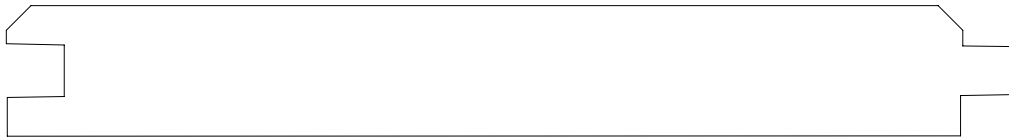
PLANKING 952521 11/16" X 5 1/4" ( 5" FACE )
