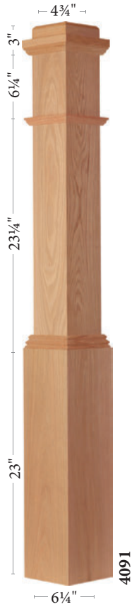
4091 POPLAR (78210) 6-1/4" x 55" Mounting Block (78211)
