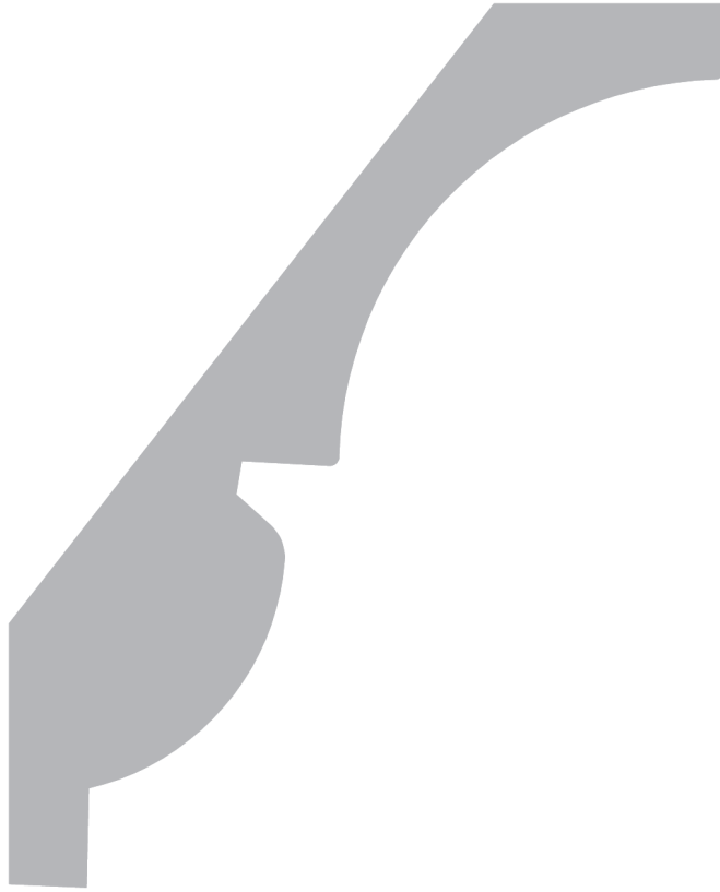
HL3532 1\frac{1}{16}'' \times 5\frac{3}{8}'' POPLAR (78827) Rise: 4" Run: 3-1/2"
