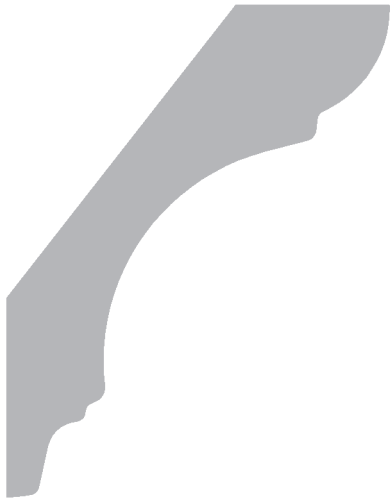
HL33251 \frac{3}{4} " x 3\frac{1}{4} " POPLAR (700366) Rise: 2-9/16" Run: 2"
